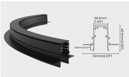
Trimless track (9.5mm(0.37") gypsum board)
