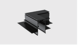
L-shaped (Downward) Model: L90-MR20(A) Material: AL6063-T5 Size: L95×W95×H46.5mm (3.74""3.74""1.83") Applicable model: TLS-MR2X0(A)
