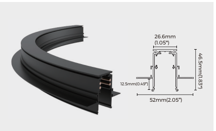
Trimless track (12.5mm gypsum board)
