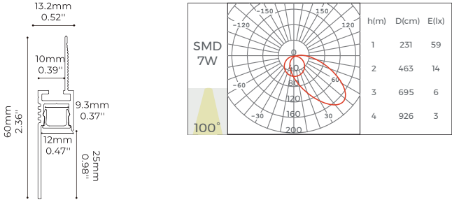
Structure image
