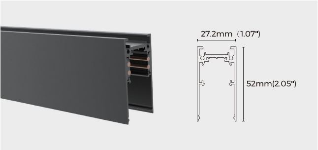
TLS-MH2X0 (X: 1 / 2 / 3 M(39.37"/78.74"/118.11")
