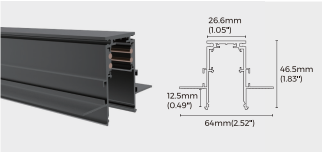
TLS-MR2X0(B) (X: 1 / 2 / 3 M(39.37"/78.74"/118.11") 12.5mm gypsum board
